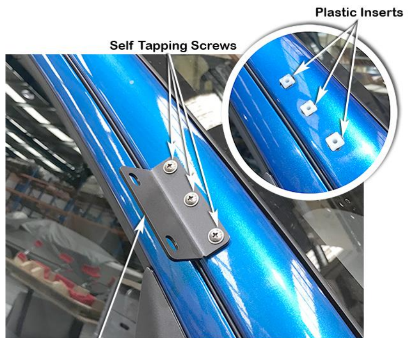
Upper Mounting Bracket
